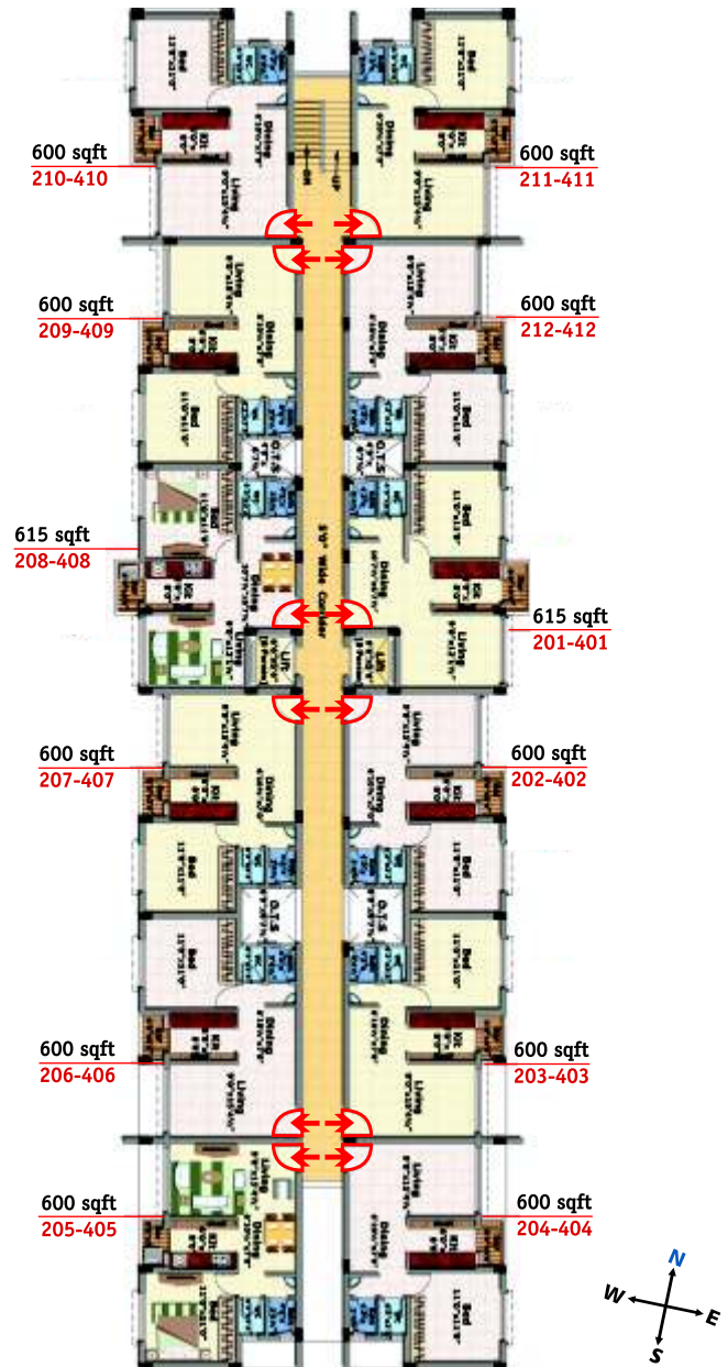
2nd, 3rd & 4th Floors
